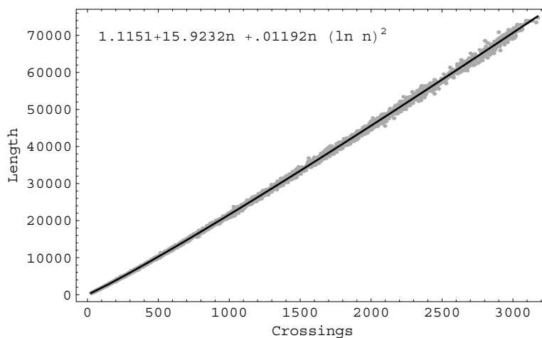
Figure 11. The length data of 2790 knots with crossing numbers ranging from 25 to 3174 together with the plot of the function y = 1.1151 + 15.9232n + 0.01192n \ln^2 n .
