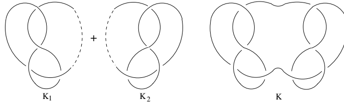
Figure 2. A composite knot K = K_1 \# K_2 .
