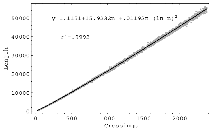
Figure 10. The evenly spread sample of 2350 knots together with the best a + bn + cn \ln^2 n fit curve, which is y = 1.1151 + 15.9232n + 0.01192n \ln^2 n with r^2 = 0.9992 . The x -axis is the crossing number of the knot and the y -axis shows the length of the cubic lattice embedding.
