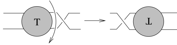
Figure 5. A single flype. T denotes a part of the diagram that is rotated by 180 degrees by the flype.
