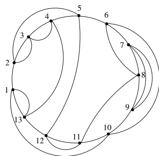
Figure 3. A small prime knot projection with 13 crossings. The Hamilton cycle is the circle and the vertices are numbered along the cycle. No “over” and “under” is indicated at the crossings.
