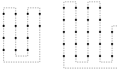
Figure 6. A planar Hamiltonian projection forming a comb with 14 or 23 vertices.
