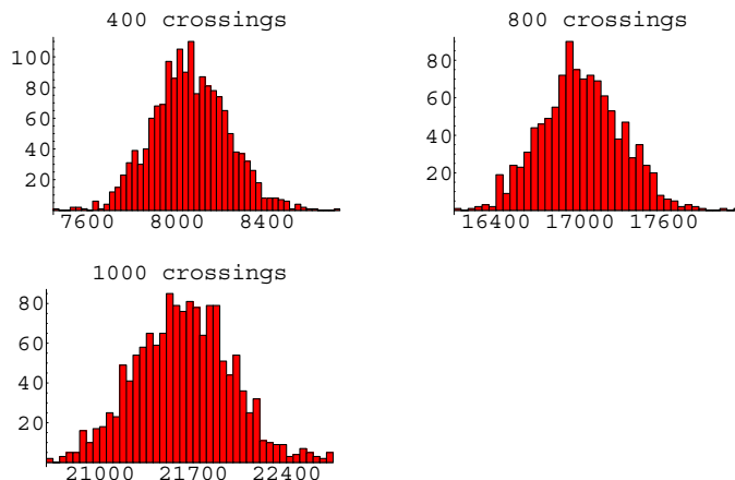
Figure 12. The embedding length distributions of the 1601 400-crossing prime knots, 1092 800-crossing prime knots and 1446 1000-crossing prime knots. The x -axis shows the embedding length and the y -axis shows the frequency of occurrences.
