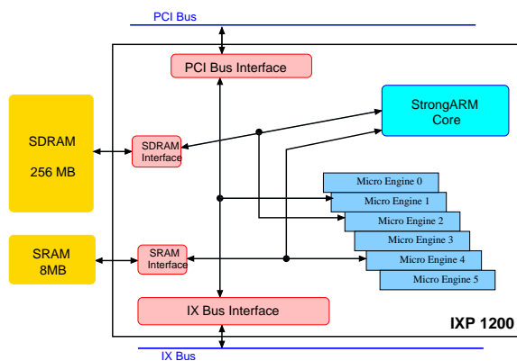
Fig. 1. IXP 1200 architecture
