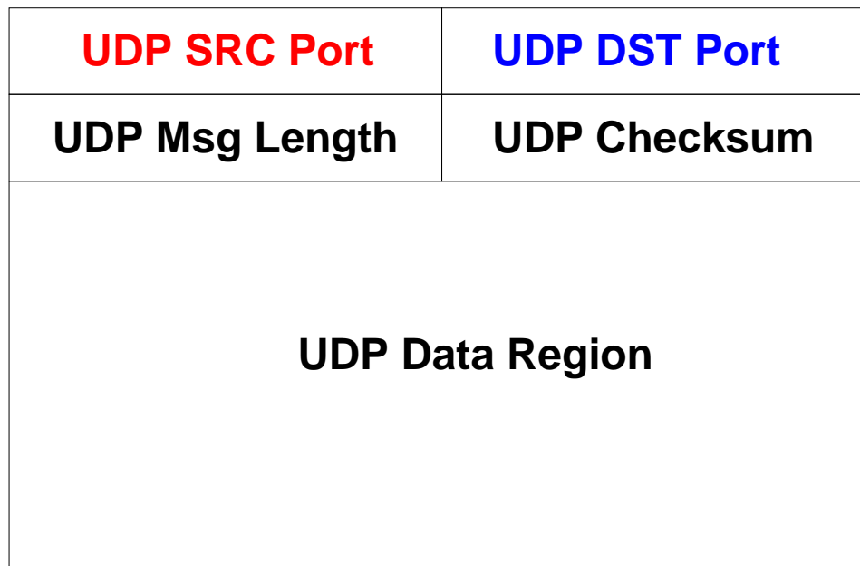
Figure 1: UDP Packet Format
